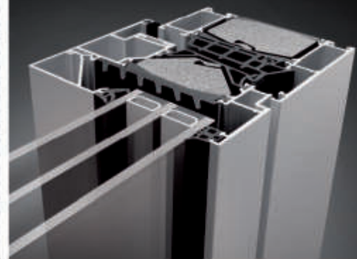
FRAME + 90 WI Aluminium-Einsatzfenster
